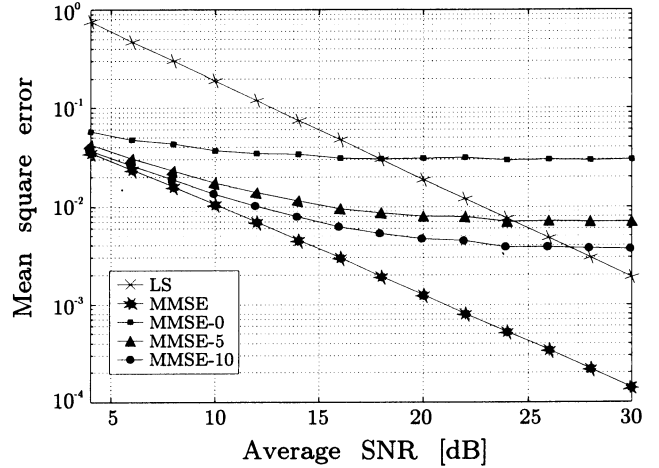
Fig. 6: Mean-square error for three modified MMSE estimators.
