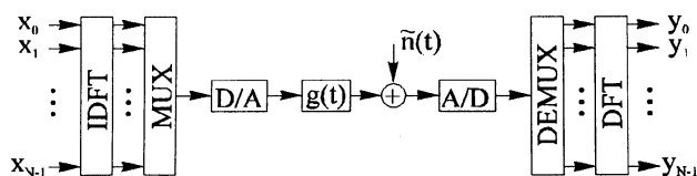
Fig. 1: Base-band OFDM system.
