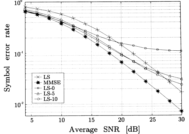
Fig. 9: Symbol error rate for three modified LS estimators.
