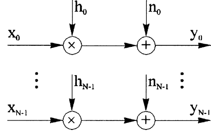
Fig. 3: Parallel Gaussian channels.
