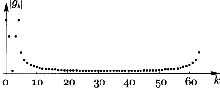
Fig. 2: Leakage between taps for the continuous channel g(t) = \delta(t - 0.5T_s) + \delta(t - 3.5T_s) .
